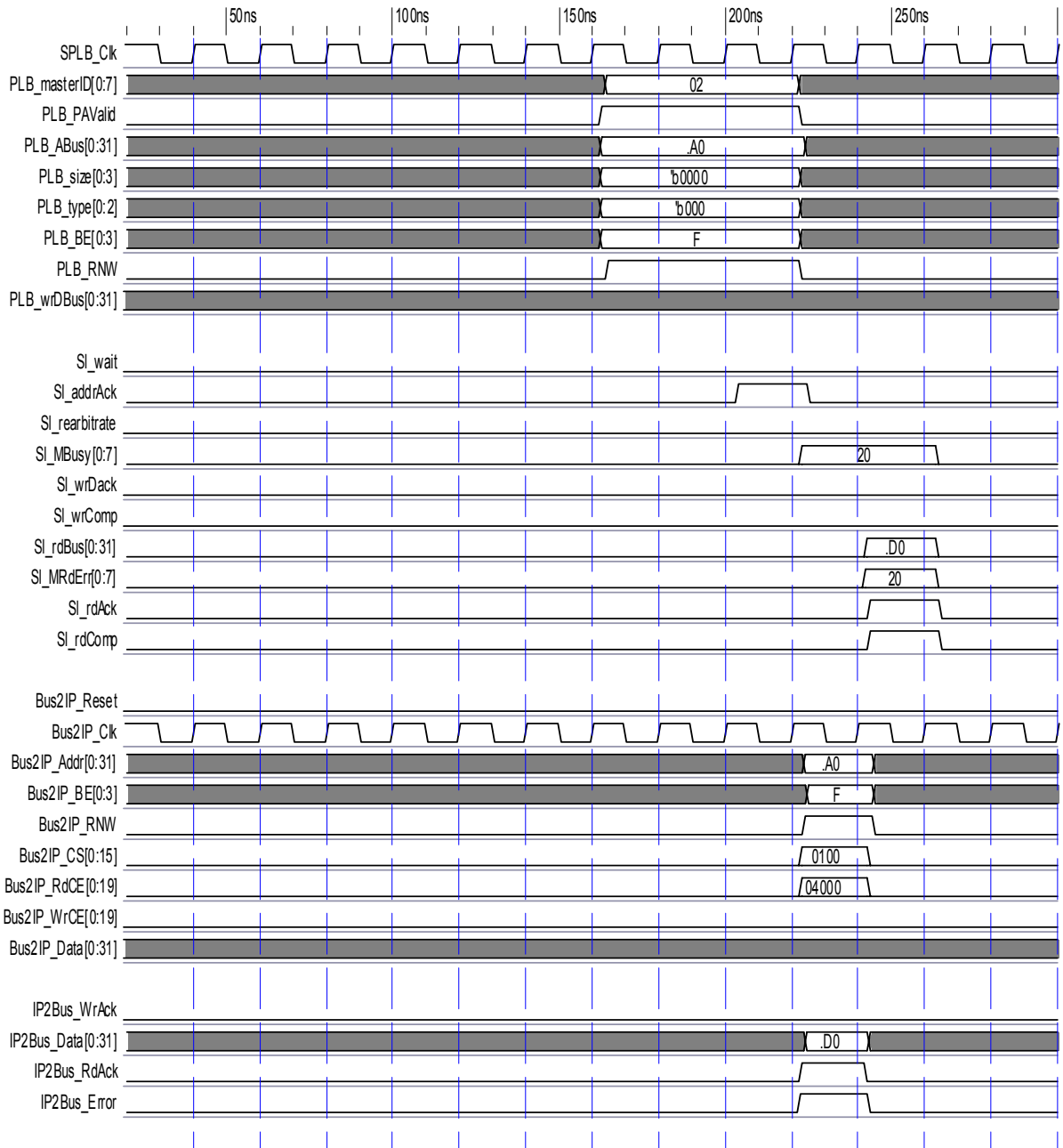
Figure 10: PLB Read Error Timing (C_SPLB_P2P=0)
